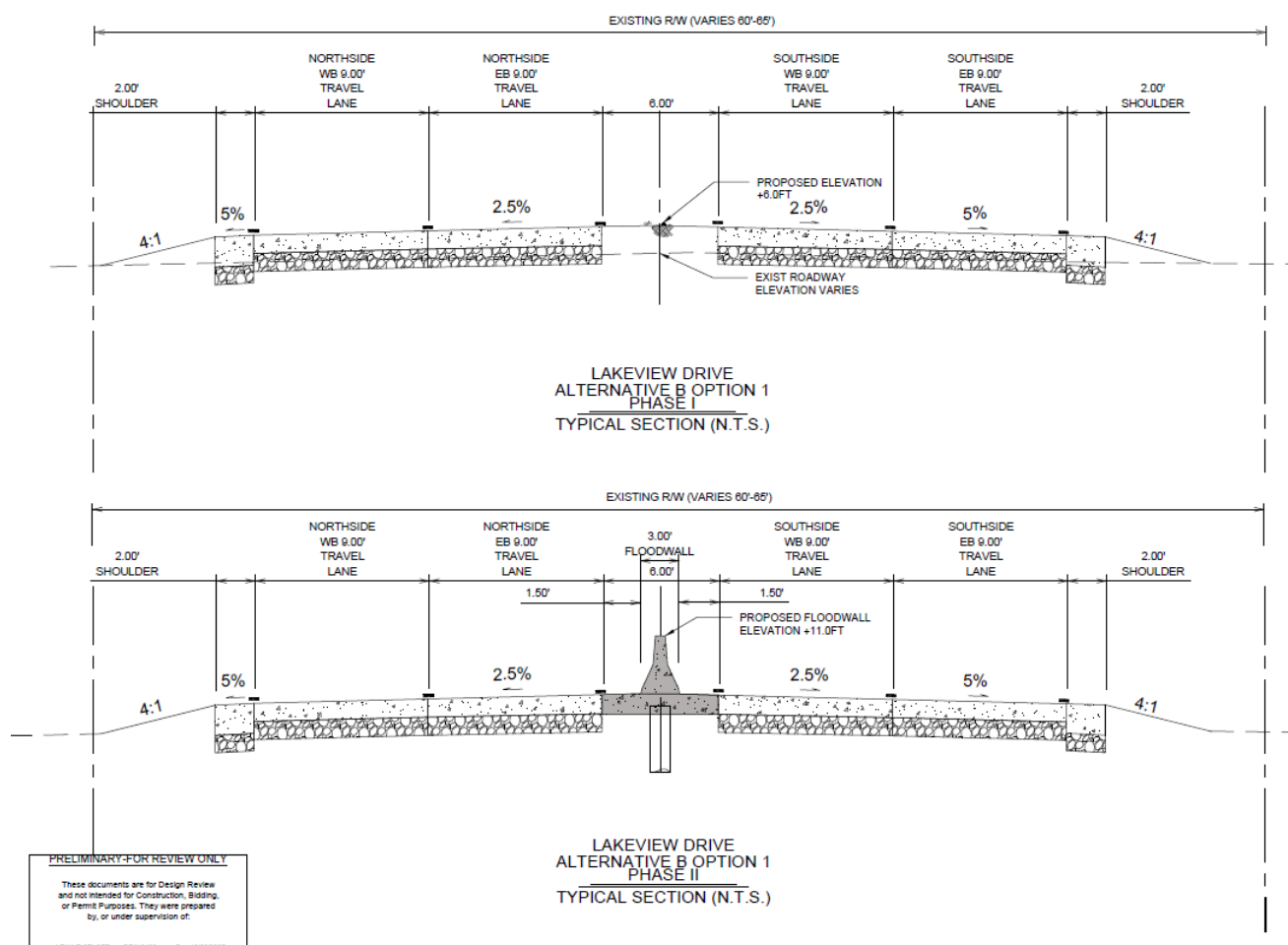
Figure 17: Alternative B, Option 1 - +6.0 ft Embankment, +11.0 ft Sheetpile Foundation Floodwall
