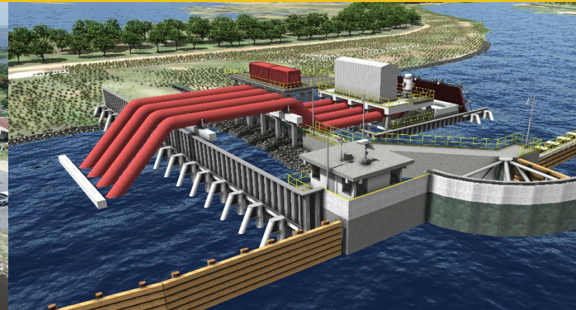
Bayou Terrebonne Pump Station 450 CFS - In Final Design
