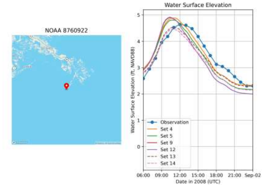
Figure 28. Hurricane Gustav modeled and observed water levels at Southwest Pass near the time of peak surge. Parameter set numbers in the figure refer to Table 3.
