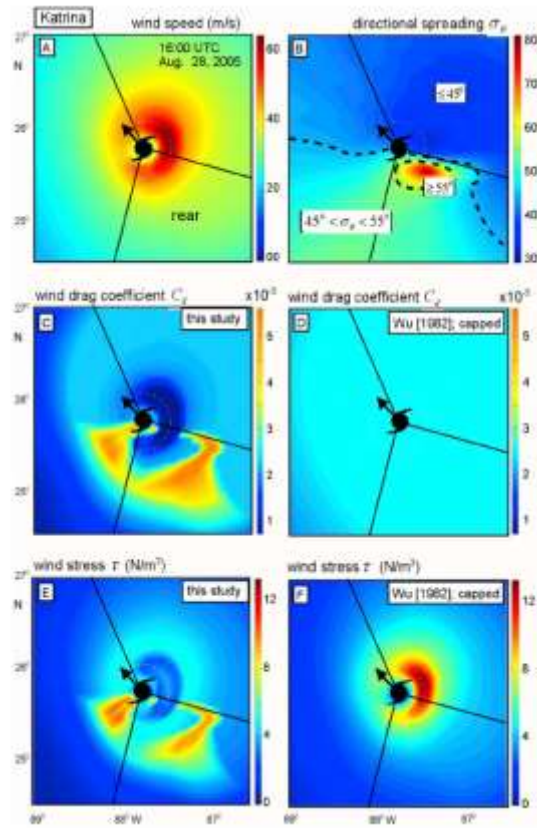
Figure 3. Patterns of wind (A), directional spread and air-sea drag (C, D) during Hurricane Katrina (Figure 10 in Holthuijsen 2012) showing the difference between the directional spreading based metric (C, E) and Wu (D, F) which very closely resembles Garratt.
