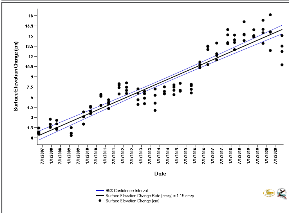
Figure A4. Examples of CRMS sites (CRMS0341 and 0178) that likely saw an acceleration in elevation gain and accretion associated with erosion into adjacent water bodies.
