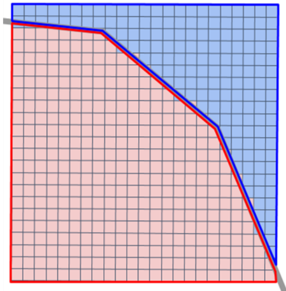
Figure 22. Relationship between ICM-Hydro compartments, ICM-Morph cells, and the proposed ICM-LAVegMod boxes. The grey line shows the boundary of an ICM-Hydro compartment; ICM-Morph cells are shown as blue and red shaded pixels; and proposed ICM-LAVegMod box boundaries are shown with darker blue and red lines.
