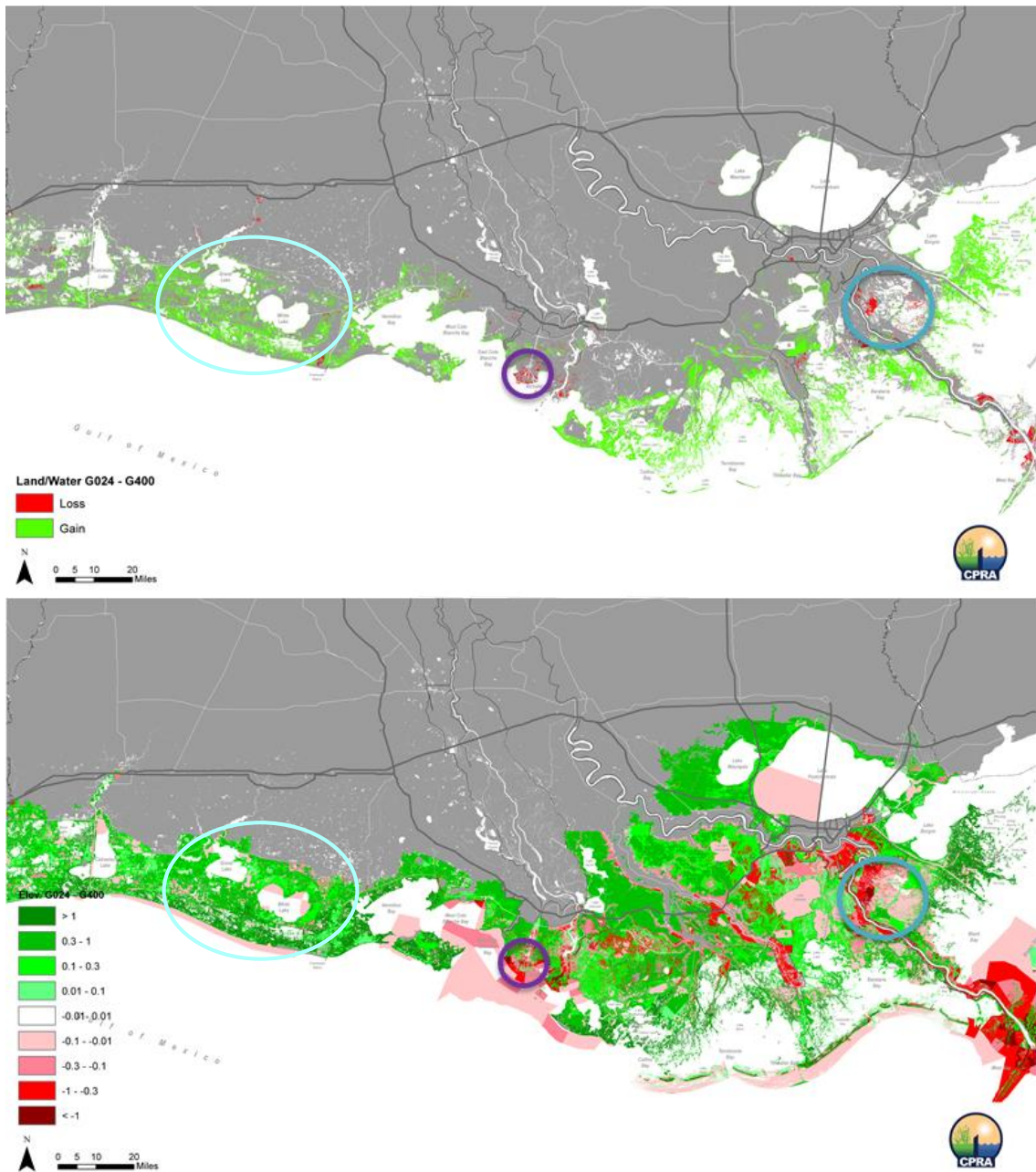
Figure G4. Land water (top) and elevation differences (bottom) between G024 and G400 at year 50. Green indicates G024>G400; red indicates G024<G400. Specific areas of interest are circled: Mermentau Basin in light blue, Wax Lake Delta in purple, and near the receiving areas for proposed Mid-Breton and Mid-Barataria sediment diversions in teal.
