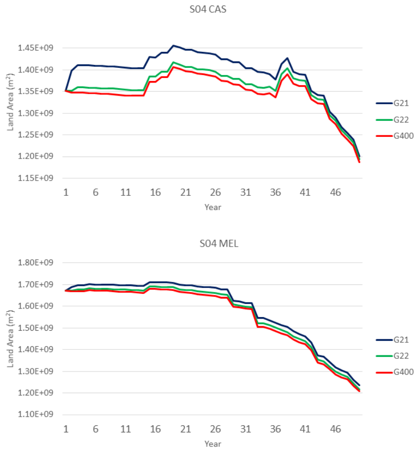
Figure D6. Land area over time for G021, G022, and the base run (G400) for example ecoregions without active 'deltaic sedimentation'. CAS – Calcasieu/Sabine. MEL – Mermentau/Lakes.
