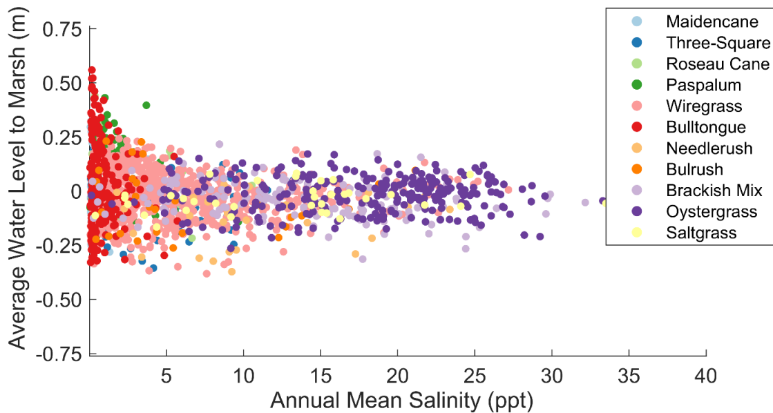
Figure 4. Water depth and salinity distribution by vegetation community in coastal Louisiana by community type. Each point represented mean salinity and depth for a single CRMS station for a single year (2010-2017), n=1944. Eleven vegetation communities are dominated by the following indicator species: Maidencane = Panicum hemitomon , Three square = Schoenoplectus americanus , Roseau cane = Phragmites australis , Paspalum = Paspalum vaginatum , Wiregrass = Spartina patens , Bulltongue = Sagittaria lancifolia , Needlerush = Juncus roemerianus , Bulrush = Bolboschoenus robustus , Oystergrass = Spartina alterniflora , Saltgrass = Distichlis spicata , and Brackish mix = none. Communities here are defined following Snedden (2019).
