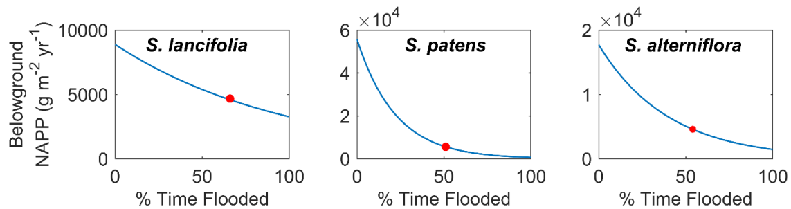
Figure 18. Belowground Net Annual Primary Production (NAPP) rates as a function of inundation duration. Rates were obtained by applying exponential regression decay parameters observed under Visser and Sandy (2009; Sagittaria lancifolia ) and Snedden et al. (2015; Spartina patens , Spartina alterniflora ). Note that Panicum hemitomon is not shown as that regression was not significant. The red dot in each regression represents the average belowground NAPP rate observed by Stagg et al. (2016), set at corresponding mean inundation rates for each marsh type.
