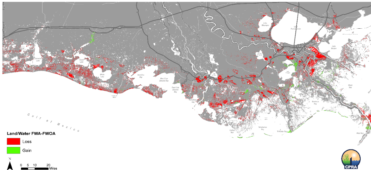
Figure C6. Land-water difference map for G020 vs. G400 at year 50.
