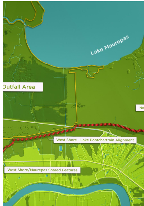
West Shore-Lake Pontchartrain HSDRRS Project
