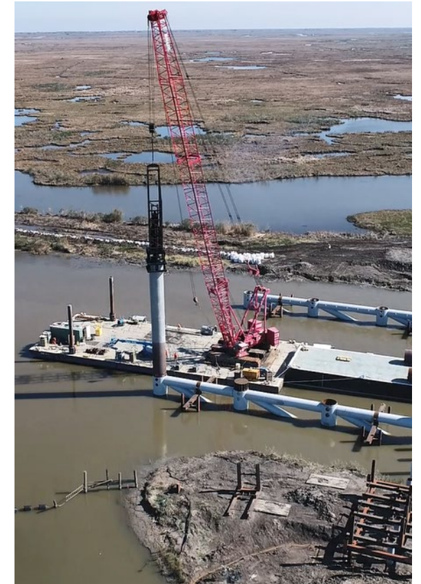
Grand Bayou Floodgate
