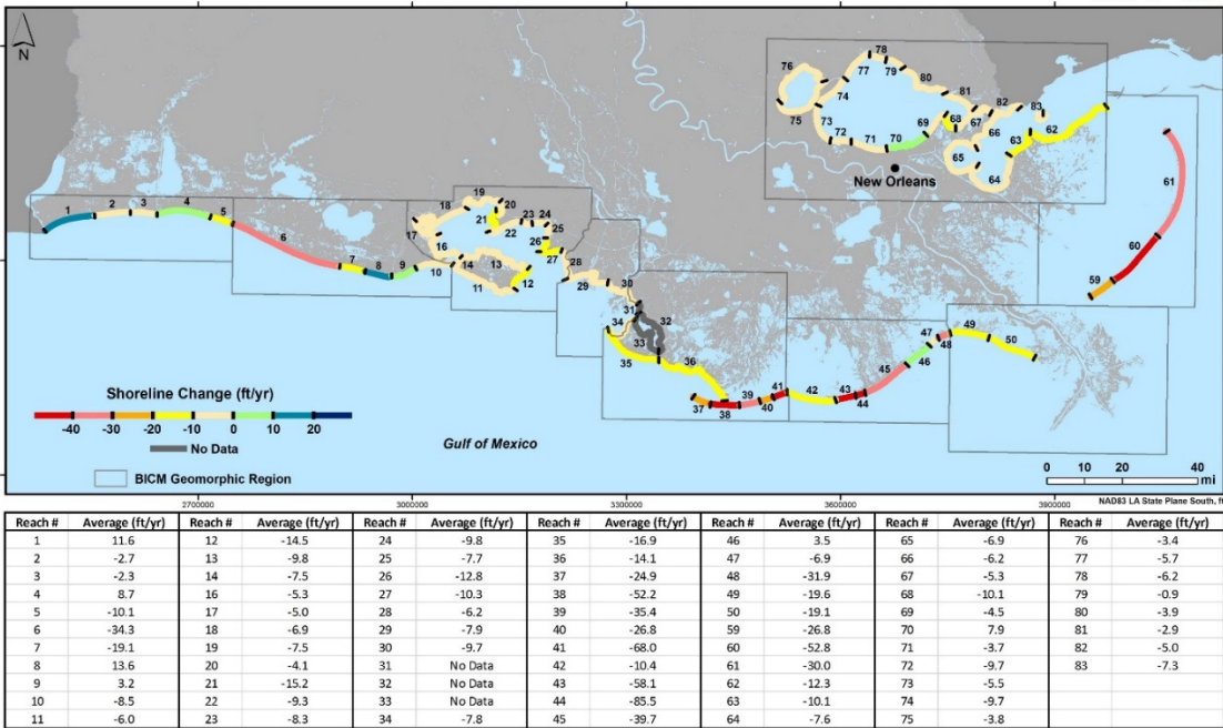
Figure 3. 1880's to 2015 average shoreline erosion rates for individual BICM shoreline reaches.
