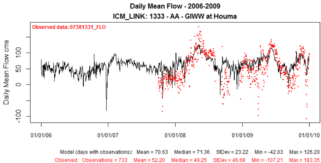
Figure 16: Modeled Flowrate at ICM Link 1333 (solid black line) Compared to Observed Data at USGS07381331 for Validation Period 2006-2009.
