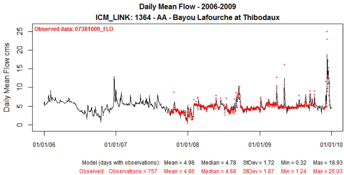
Figure 22: Modeled Flowrate at ICM Link 1364 (solid black line) Compared to Observed Data at USGS07381000 for Validation Period 2006-2009.
