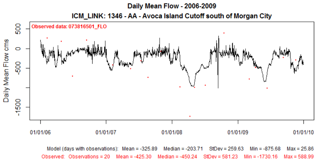
Figure 18: Modeled Flowrate at ICM Link 1346 (solid black line) Compared to Observed Data at USGS073816501 for Validation Period 2006-2009.
