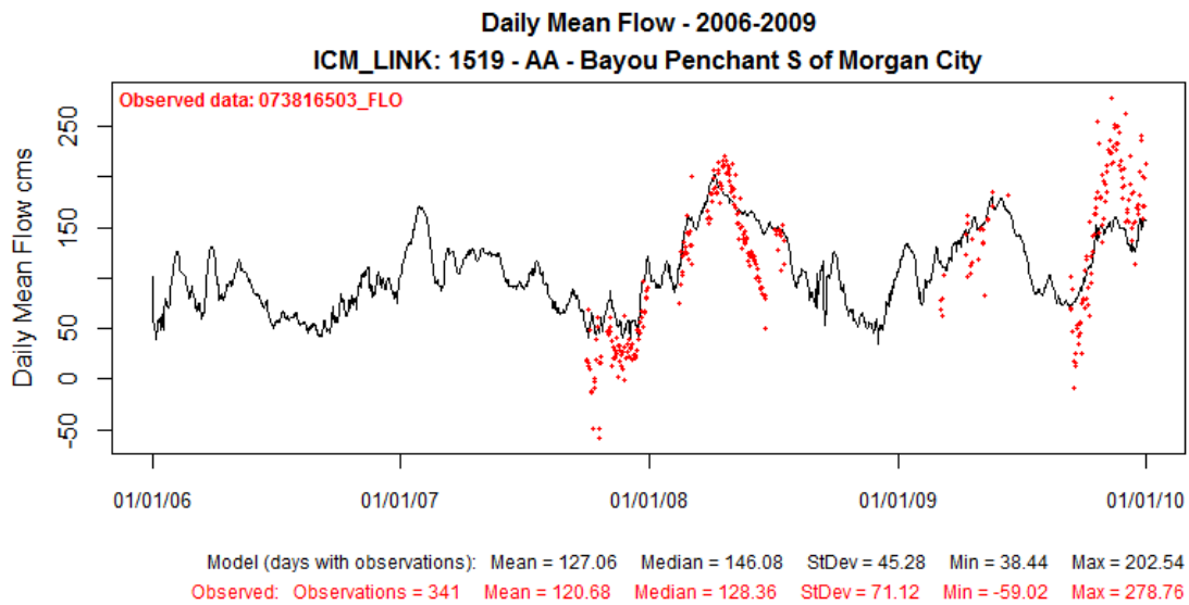
Figure 24: Modeled Flowrate at ICM Link 1519 (solid black line) Compared to Observed Data at USGS073816503 for Validation Period 2006-2009.
