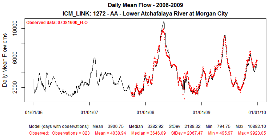
Figure 6: Modeled Flowrate at ICM Link 1272 (solid black line) Compared to Observed Data at USGS07381600 for Validation Period 2006-2009.
