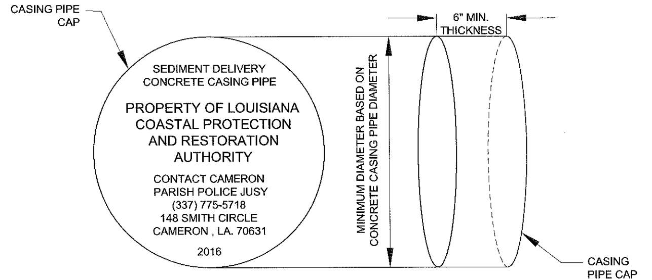
CASING PIPE CAP DETAIL (NOT TO SCALE)
