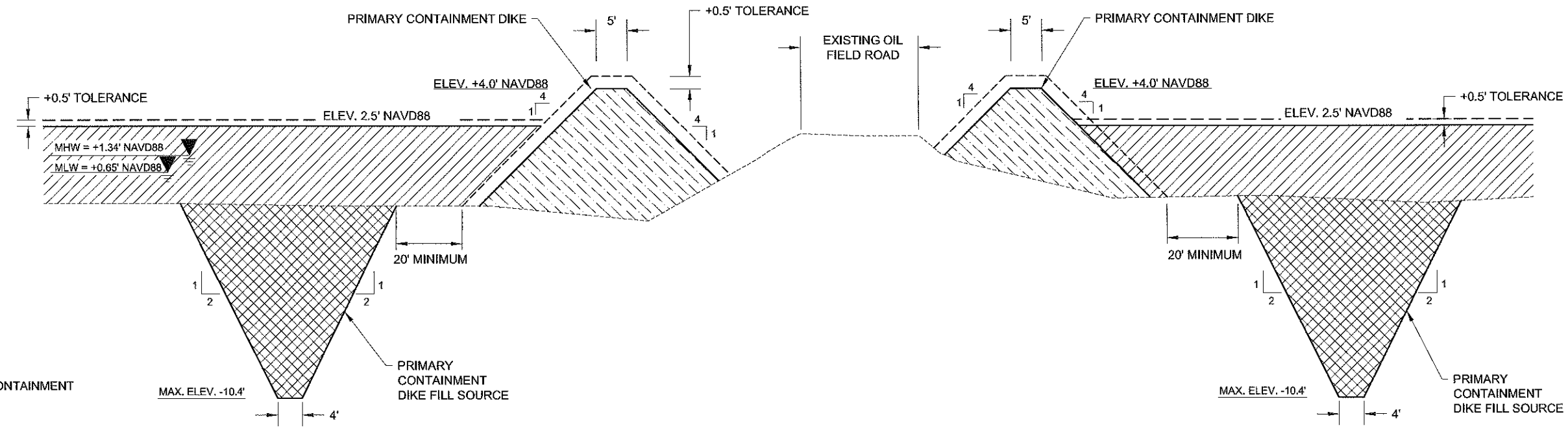
TYPICAL PRIMARY CONTAINMENT DIKE ADJACENT TO EXISTING OIL FIELD ROAD (STA. 55+00) NOT TO SCALE
