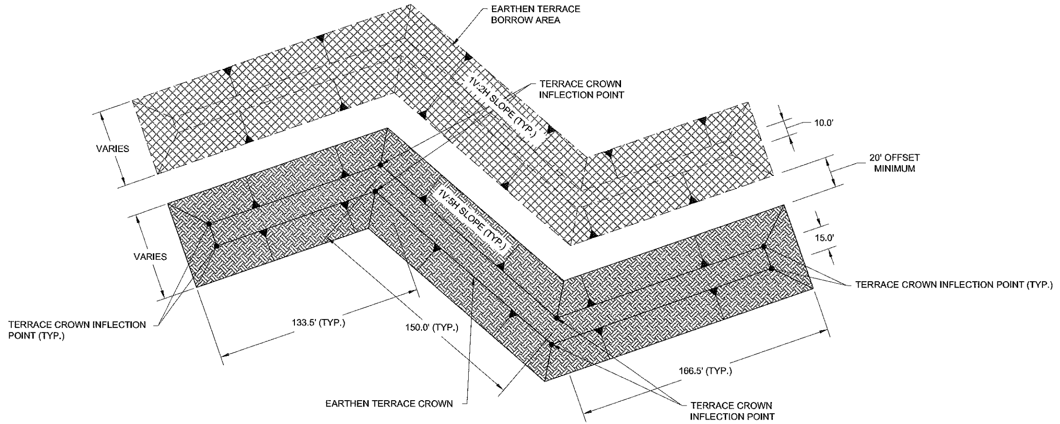
TYPICAL EARTHEN TERRACE DETAIL PLAN VIEW
