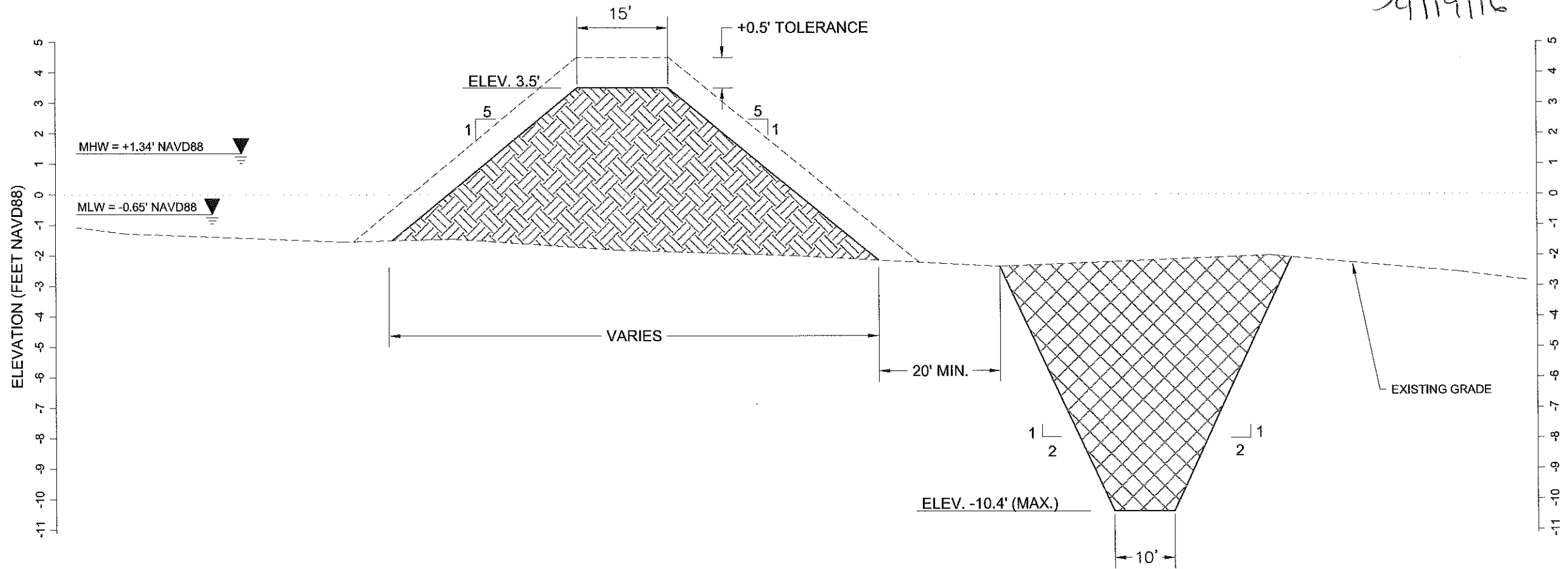
TYPICAL EARTHEN TERRACE CROSS SECTION
