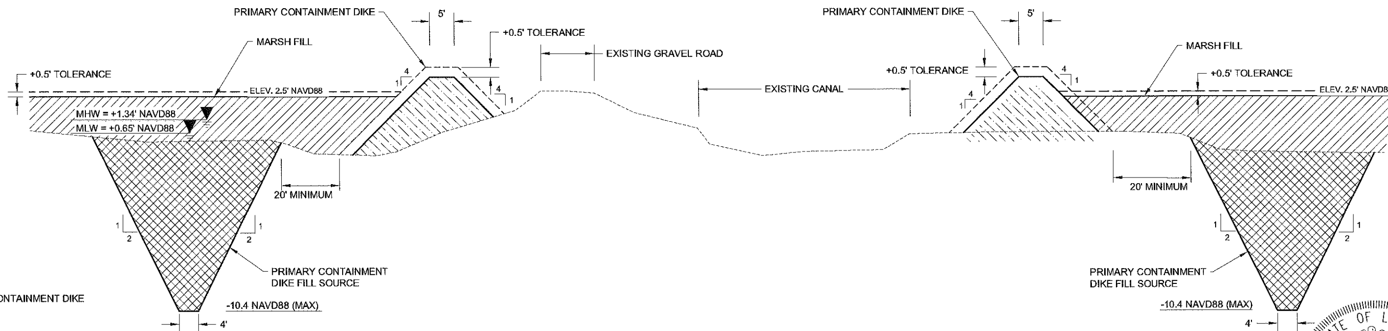
TYPICAL PRIMARY CONTAINMENT DIKE NEAR CANAL STA. 80+00 NOT TO SCALE
