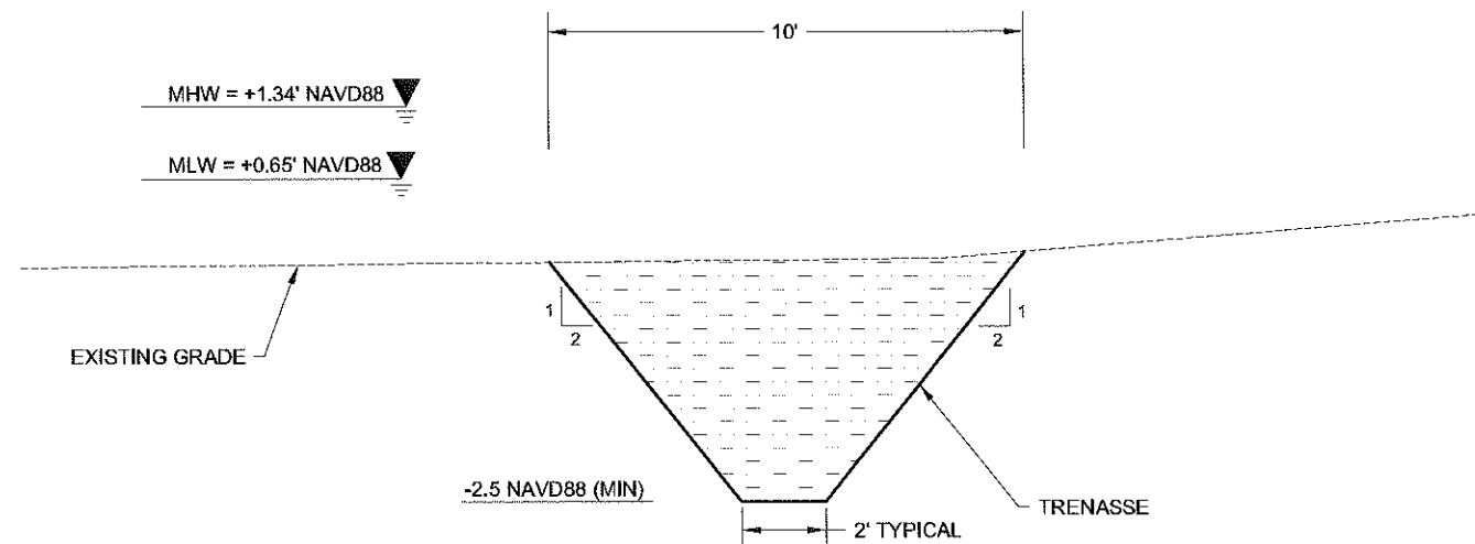
TRENASSE TYPICAL SECTION NOT TO SCALE
