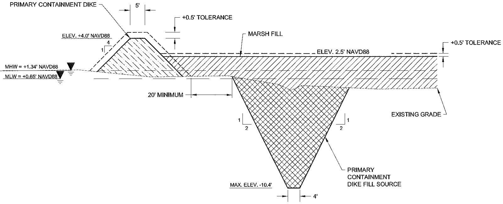
TYPICAL PRIMARY CONTAINMENT DIKE SECTION NOT TO SCALE
