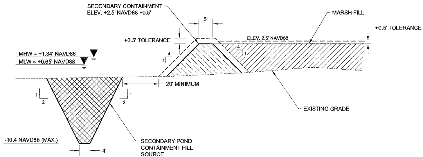
TYPICAL SECONDARY POND CONTAINMENT TYPICAL SECTION NOT TO SCALE
