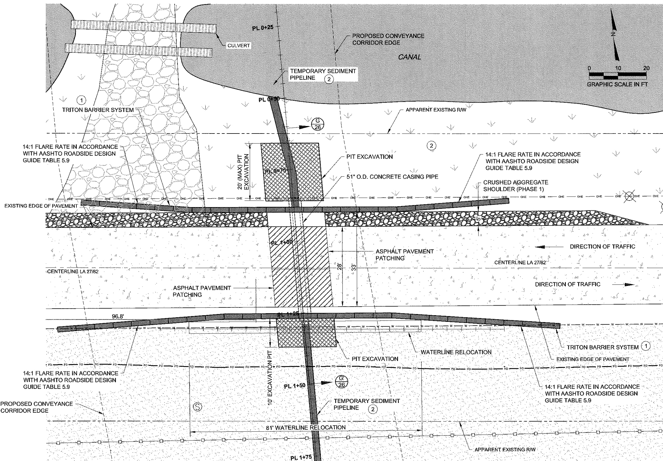
PLAN VIEW
