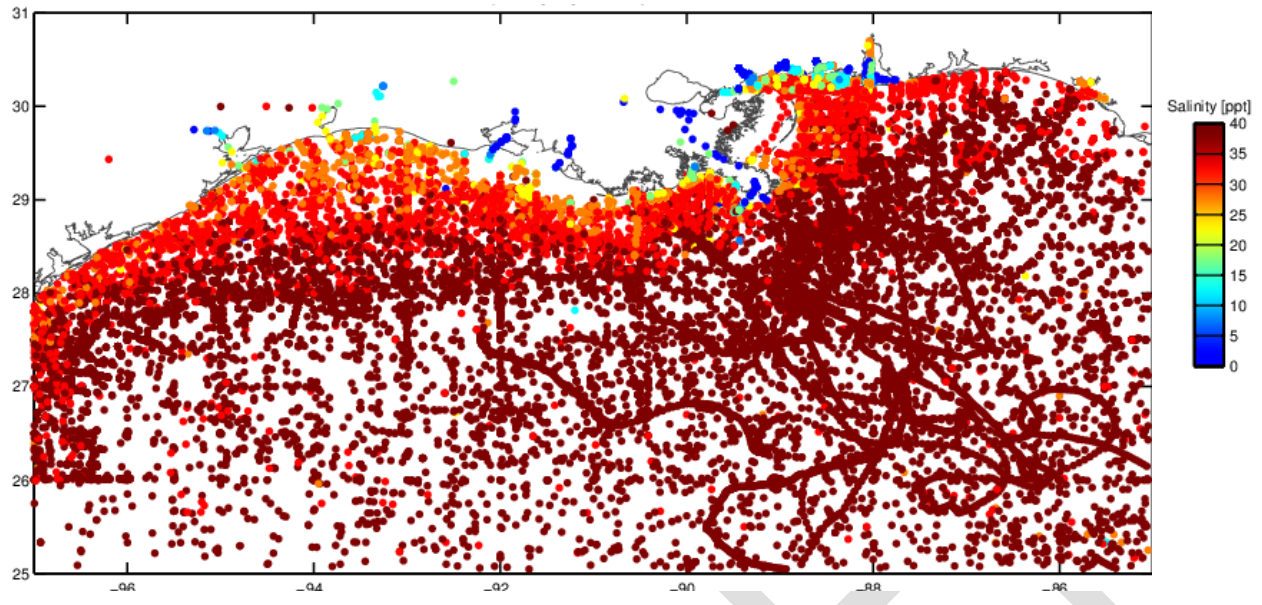
Figure 9: WOD Salinity Data.
