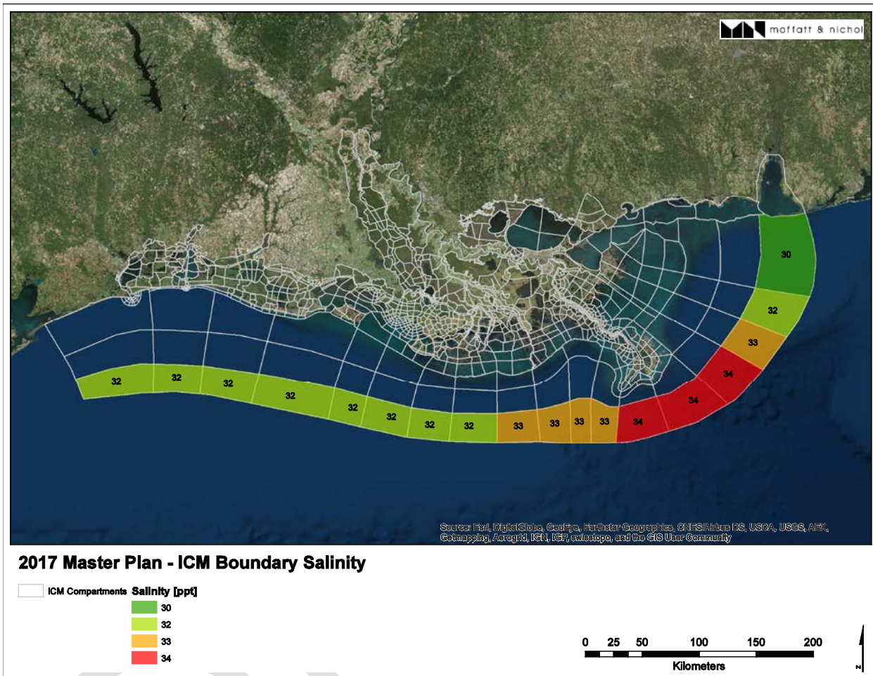
Figure 13: ICM Boundary Compartment Salinity.
