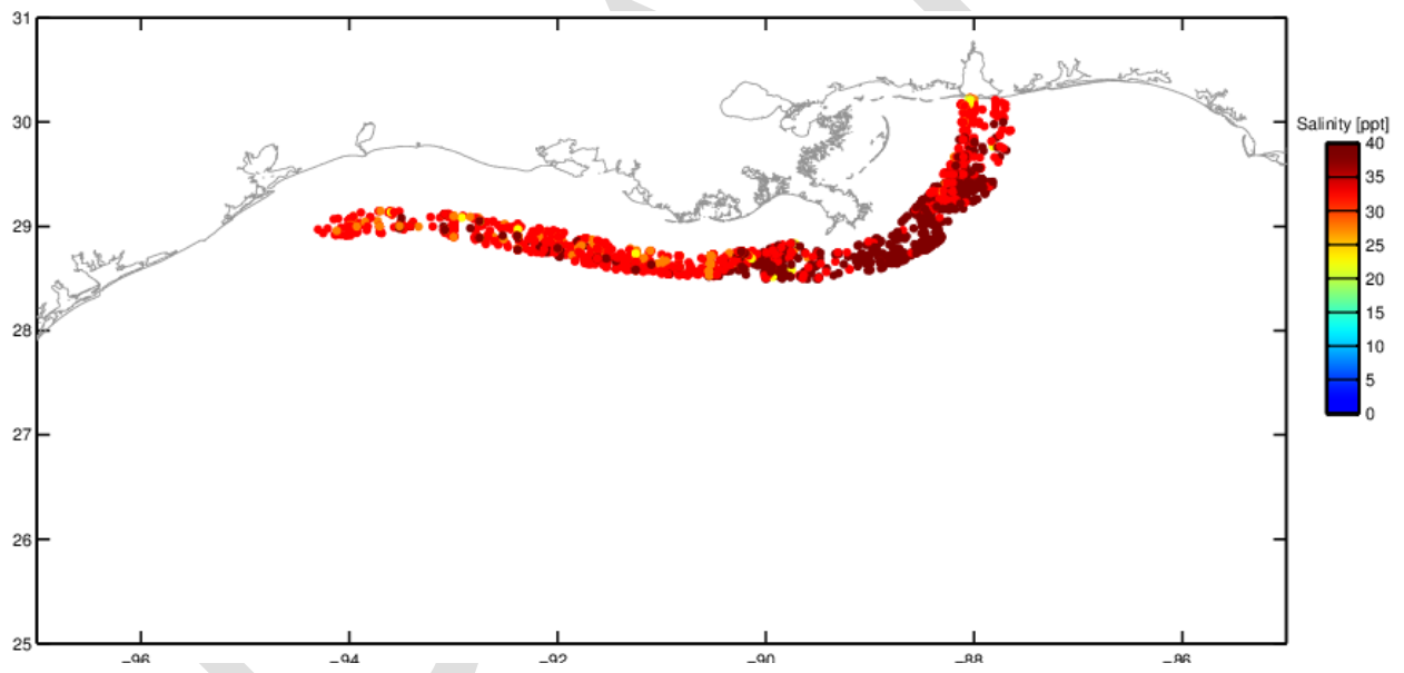
Figure 10: WOD Salinity Data inside ICM Boundary Compartments.
