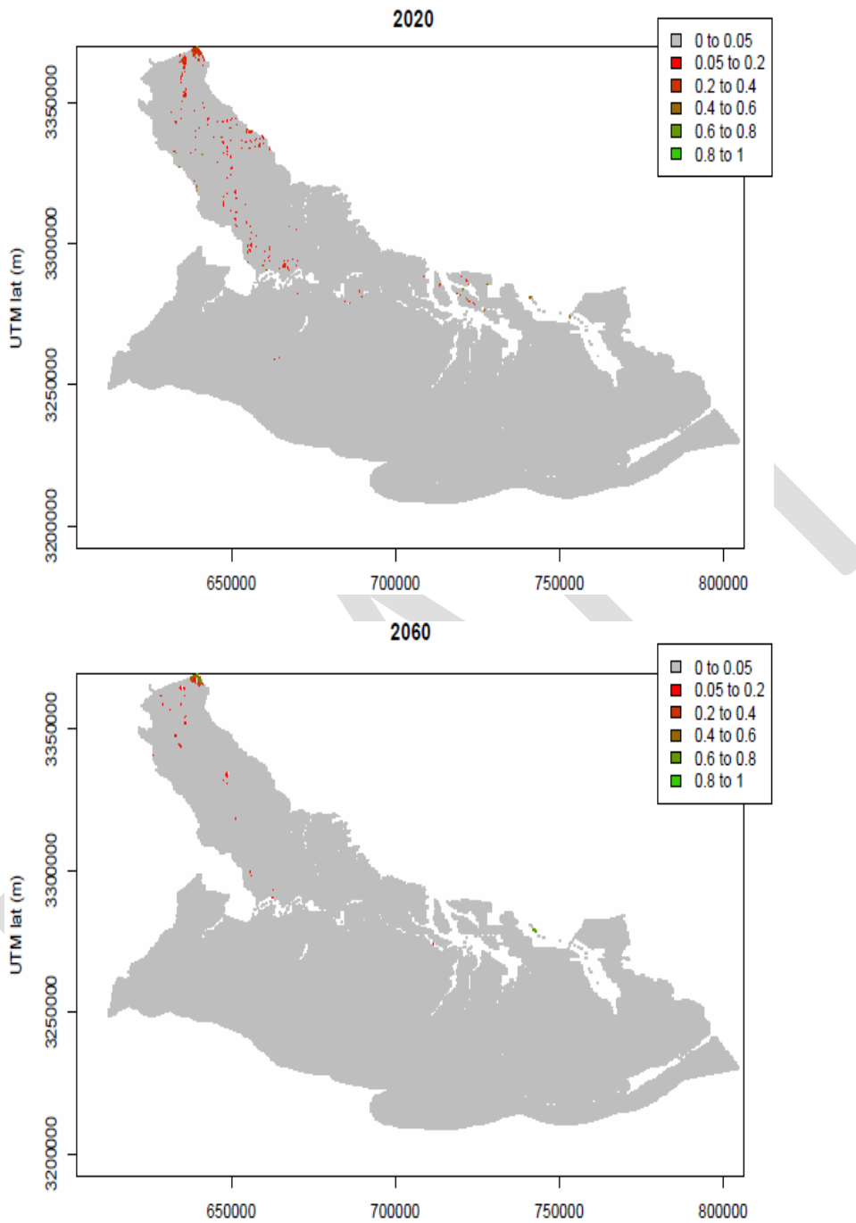
Figure 7.15. Distribution of Quercus nigra in years 2020 (top) and 2060 (bottom). Areas are colored from red to green based on the fraction of a cell covered. Red indicates low cover (0.05 to 0.2), bright green indicates high cover (0.8 and 1.0). Cover is indicated by the fraction of each 500x500 m cell occupied by a species.
