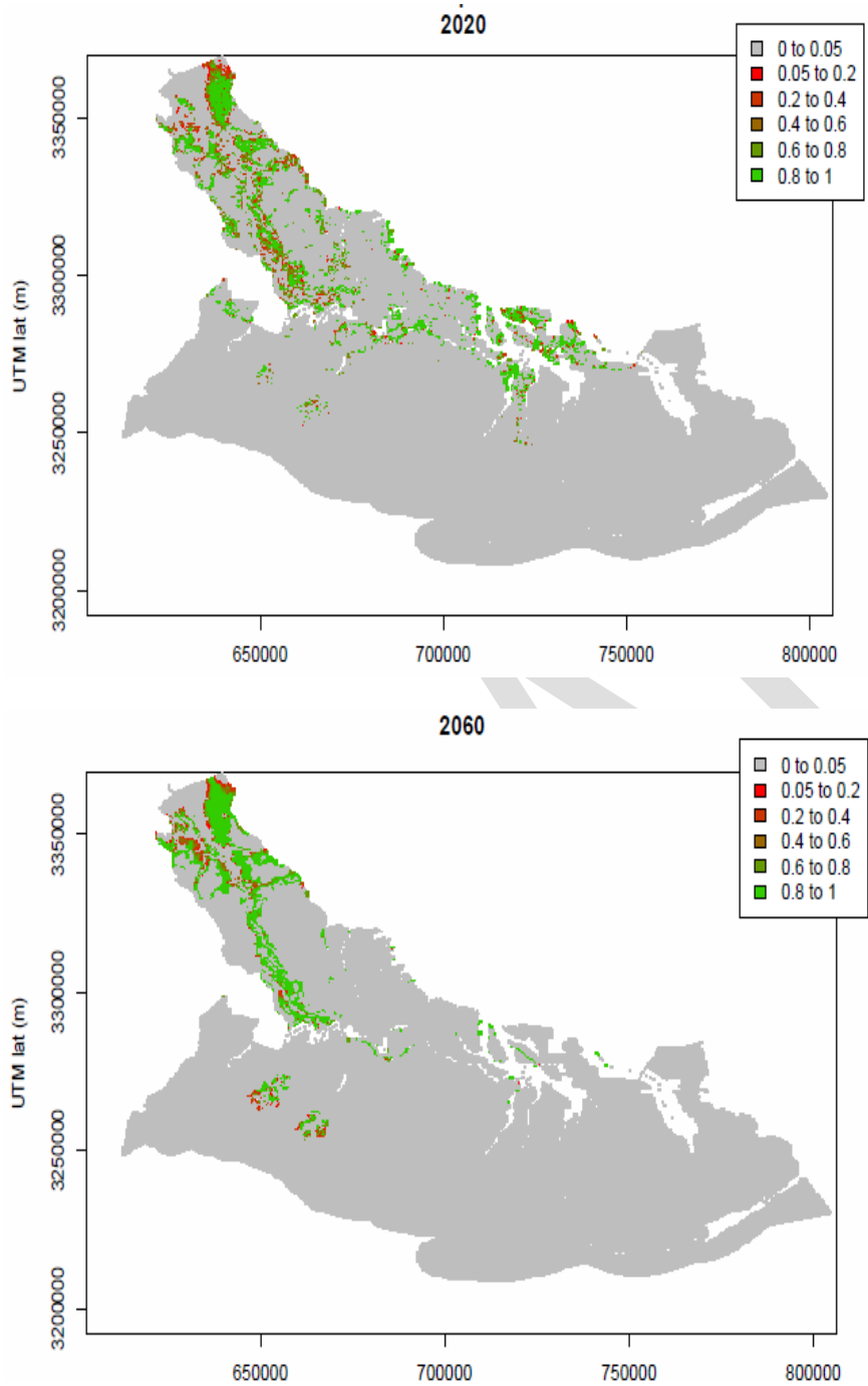
Figure 7.13. Distribution of Quercus lyrata in years 2020 (top) and 2060 (bottom). Areas are colored from red to green based on the fraction of a cell covered. Red indicates low cover (0.05 to 0.2), bright green indicates high cover (0.8 and 1.0). Cover is indicated by the fraction of each 500x500 m cell occupied by a species.
